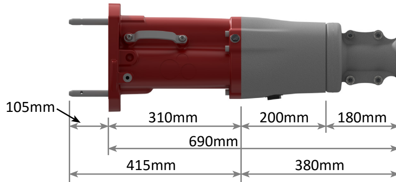
Side View (UN-ARM)
