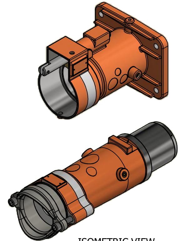
ISOMETRIC VIEW PLUG & RECEPTACLE 660V 425A 4 PIN
